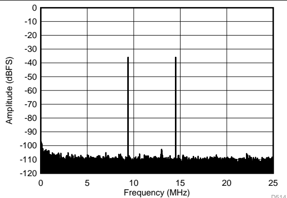
f_{IN1} = 185 \text{ MHz} , f_{IN2} = 190 \text{ MHz} , \text{IMD3} = 85 \text{ dBFS} , each tone at -36 dBFS
