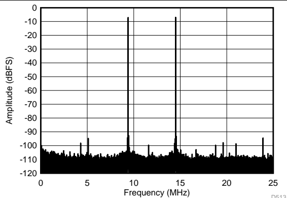
f_{IN1} = 185 \text{ MHz} , f_{IN2} = 190 \text{ MHz} , \text{IMD3} = 83 \text{ dBFS} , each tone at -7 dBFS
