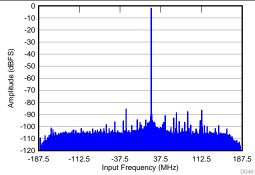
f_{IN} = 1.78 \text{ GHz} , A_{IN} = -2 \text{ dBFS} , f_S = 2949.12 \text{ MSPS} , SNR = 62.6 dBFS, SFDR (includes IL) = 86 dBc
