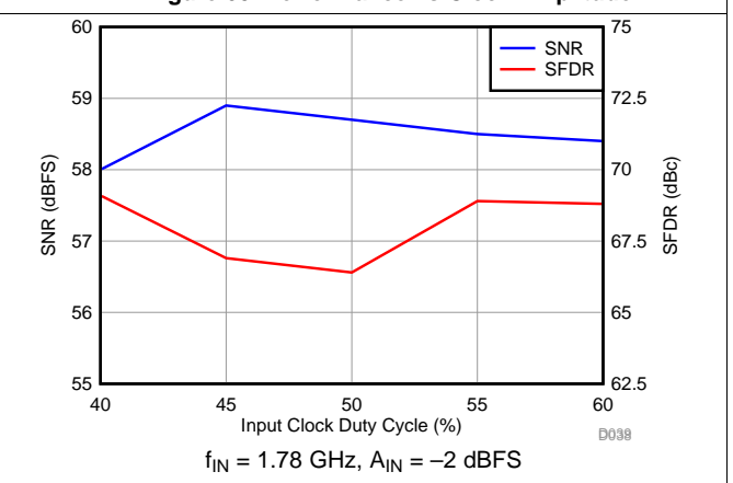
Figure 62. Performance vs Clock Duty Cycle
