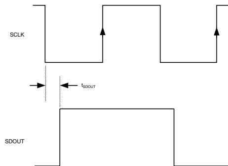
Figure 136. SDOUT Timing
