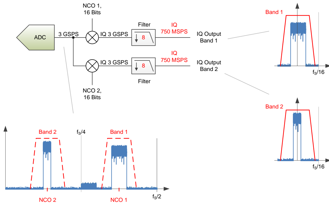
Figure 96. Dual-Band Example
