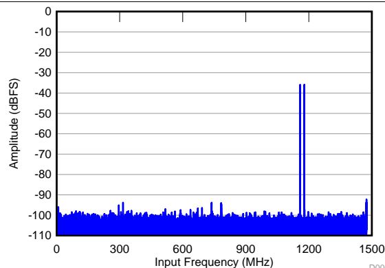
f_{IN1} = 1.77 \text{ GHz} , f_{IN2} = 1.790 \text{ GHz} , A_{IN} = -36 \text{ dBFS} , \text{IMD} = 97 \text{ dBFS}
