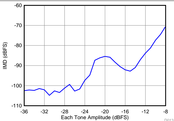
f_{IN1} = 1.77 GHz, f_{IN2} = 1.79 GHz
