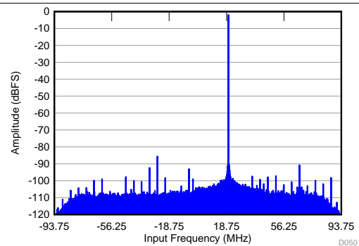
f_{IN} = 1.78 \text{ GHz} , A_{IN} = -2 \text{ dBFS} , f_S = 2949.12 \text{ MSPS} , SNR = 63.9 dBFS, SFDR (includes IL) = 83 dBc
