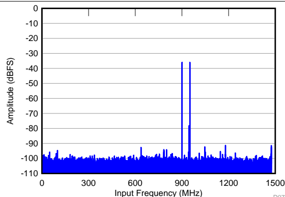
f_{IN1} = 900 \text{ MHz} , f_{IN2} = 950 \text{ MHz} , A_{IN} = -36 \text{ dBFS} , \text{IMD} = 97 \text{ dBFS}
