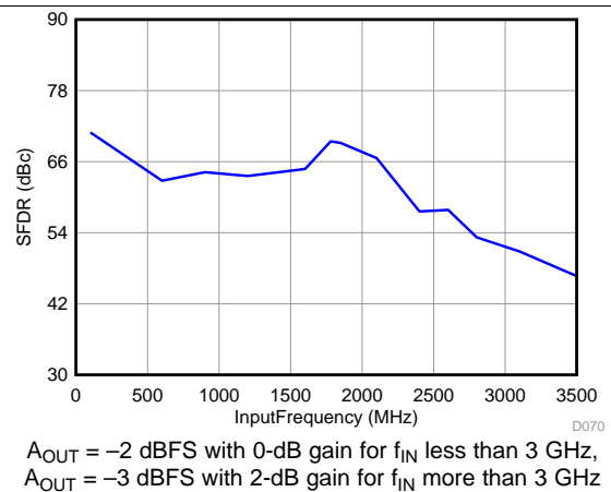
Figure 38. Spurious-Free Dynamic Range vs Input Frequency ( f_s = 2457.6 MSPS)
