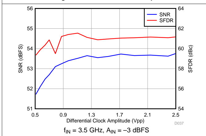
Figure 61. Performance vs Clock Amplitude
