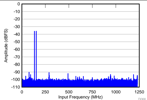
f_{IN1} = 2.59 GHz, f_{IN2} = 2.6 GHz, A_{IN} = -36 dBFS, IMD = 92 dBFS
