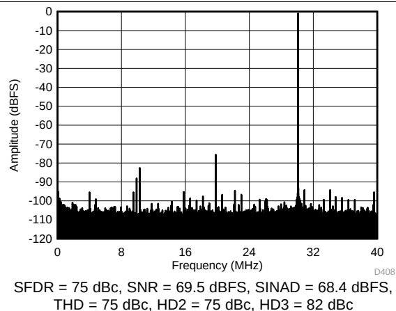
Figure 68. FFT for 270-MHz Input Signal (Dither Off)
