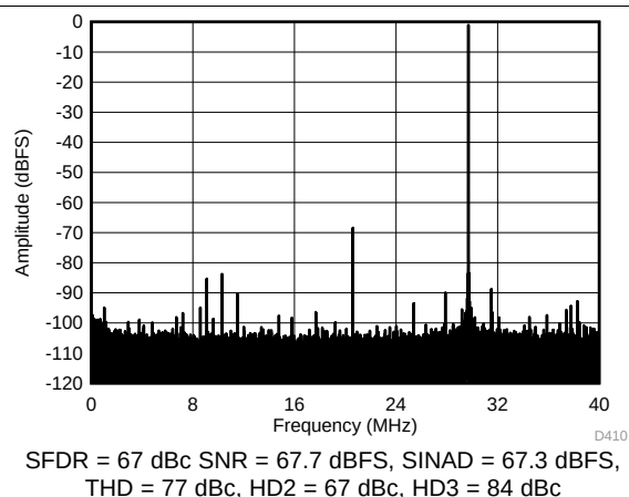
Figure 70. FFT for 450-MHz Input Signal (Dither Off)
