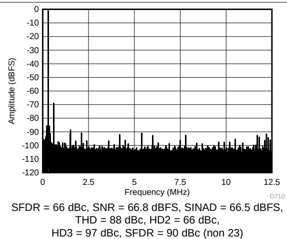
Figure 10. FFT for 450-MHz Input Signal (Dither Off)
