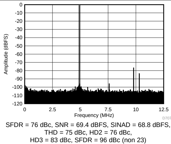
Figure 7. FFT for 270-MHz Input Signal (Dither On)
