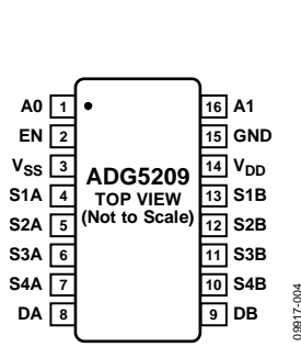
Figure 4. ADG5209 Pin Configuration (TSSOP)
