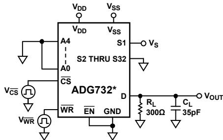
Figure 29. Write Turn-On and Turn-Off Time, t_{ON}, t_{OFF}(\overline{WR})
