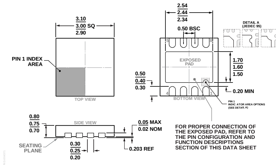
Figure 70. 8-Lead Lead Frame Chip Scale Package [LFCSP] 3 mm x 3 mm Body and 0.75 mm Package Height (CP-8-21)
