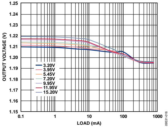
Figure 16. Load Regulation, V_{OUT} = 1.2V
