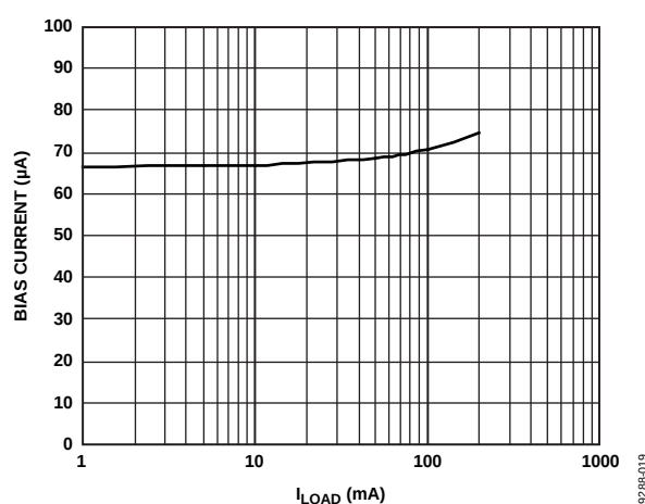
Figure 21. Bias Current vs. Load Current, Single Output Loaded, V_{\text{RIPPLE}} = 50 \text{ mV} , C_{\text{OUT}} = 1 \mu\text{F}
