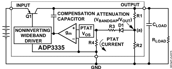
Figure 23. Functional Block Diagram
