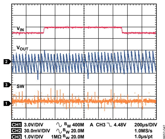
Figure 42. Buck Response to Line Transient, Input Voltage from 4.5\text{ V} to 5.0\text{ V} , V_{OUT1} = 1.8\text{ V} , I_{OUT1} = 5\text{ mA} , Auto Mode
