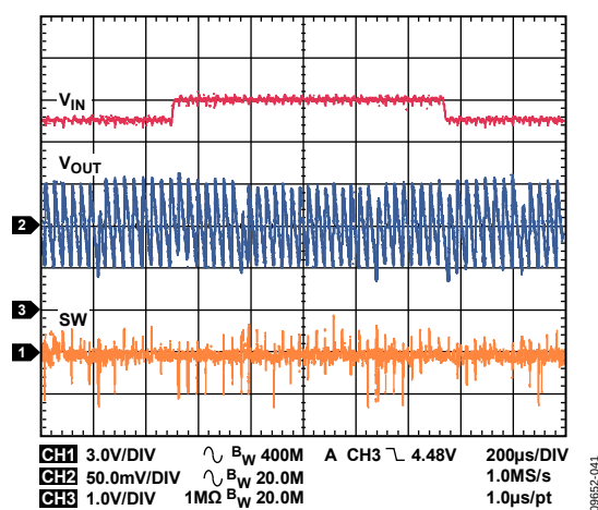
Figure 41. Buck Response to Line Transient, Input Voltage from 4.5\text{ V} to 5.0\text{ V} , V_{OUT1} = 3.3\text{ V} , I_{OUT1} = 5\text{ mA} , Auto Mode
