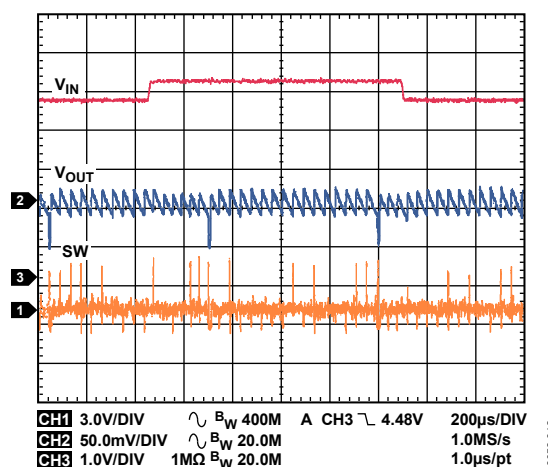
Figure 43. Buck Response to Line Transient, Input Voltage from 4.5\text{ V} to 5.0\text{ V} , V_{OUT1} = 1.2\text{ V} , I_{OUT1} = 5\text{ mA} , Auto Mode
