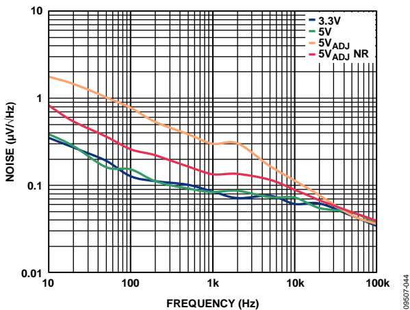
Figure 49. Output Noise Spectral Density, I_{LOAD} = 10\text{ mA} , C_{OUT} = 1\ \mu\text{F}
