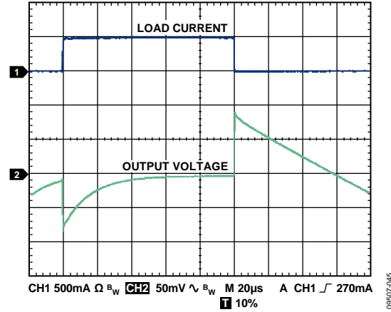
Figure 50. Load Transient Response, C_{IN}, C_{OUT} = 1\ \mu\text{F} , I_{LOAD} = 1\text{ mA to } 500\text{ mA} , V_{OUT} = 1.8\text{ V} , V_{IN} = 5\text{ V}
