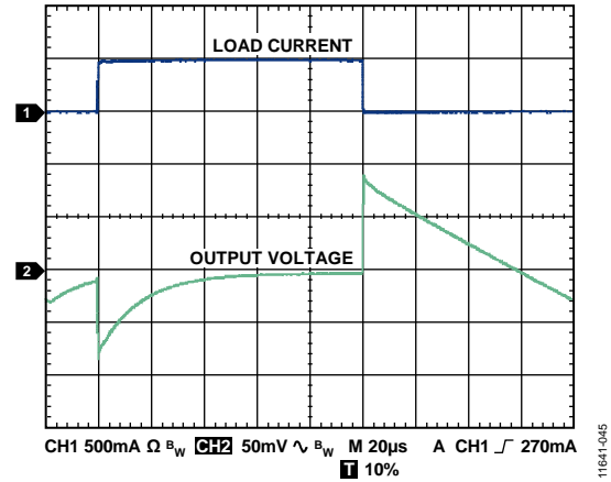
Figure 51. Load Transient Response, C_{IN} = C_{OUT} = 1 \mu F , I_{LOAD} = 1 mA to 500 mA , V_{OUT} = 1.8 V , V_{IN} = 5 V
