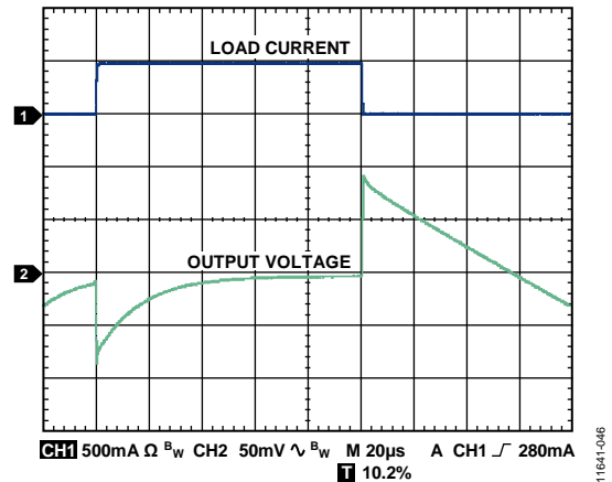
Figure 52. Load Transient Response, C_{IN} = C_{OUT} = 1 \mu F , I_{LOAD} = 1 mA to 500 mA , V_{OUT} = 3.3 V , V_{IN} = 5 V
