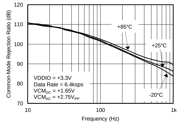
Figure 12. CMRR vs Frequency
