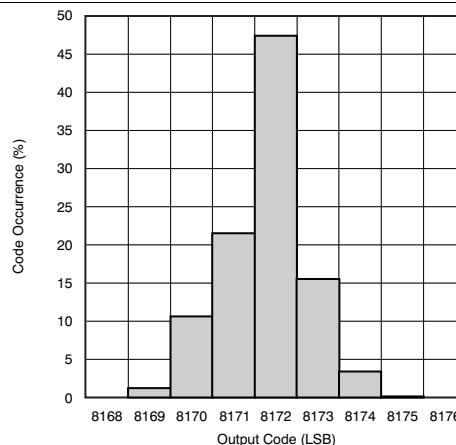
Figure 62. Output Noise Histogram (With Inputs Shorted to VCM)
