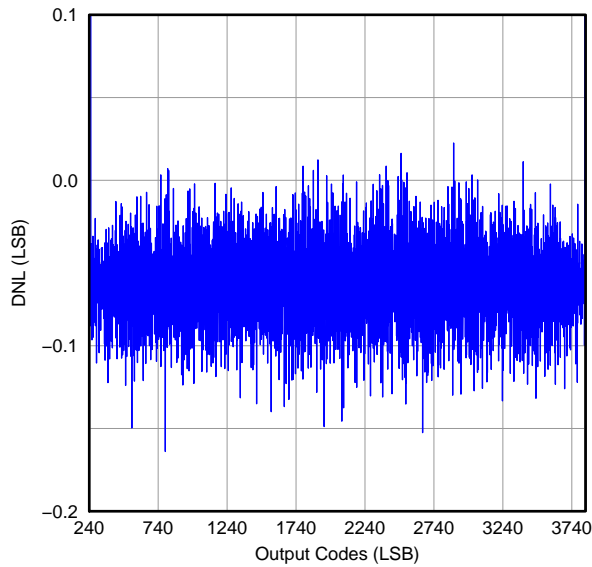
Figure 28. Differential Non-Linearity
