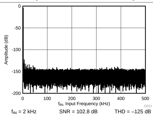
Figure 21. Typical FFT
