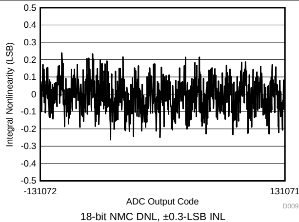
Figure 104. Typical Linearity
