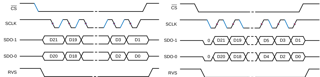
Figure 62. SPI-10-D Protocol
