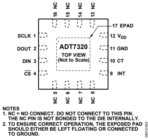
Figure 3. Pin Configuration
