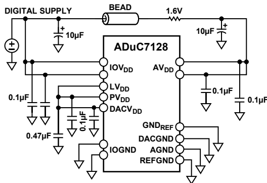
Figure 67. External Single Supply Connections
