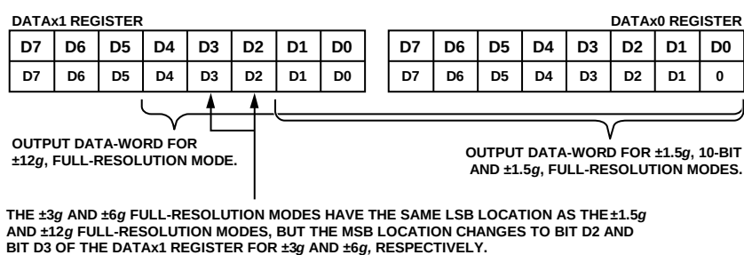
Figure 33. Data Formatting of Full-Resolution and \pm 1.5 g, 10-Bit Modes of Operation When Output Data Is Right Justified
