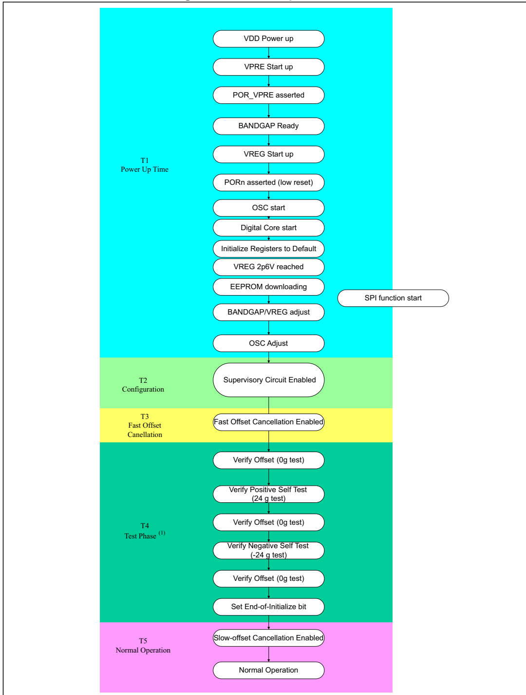
Figure 17. Power-up flowchart
