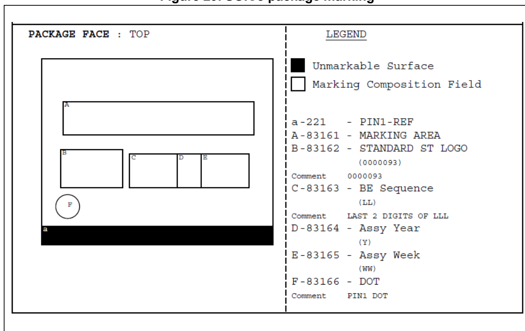
Figure 29. SOIC8 package marking
