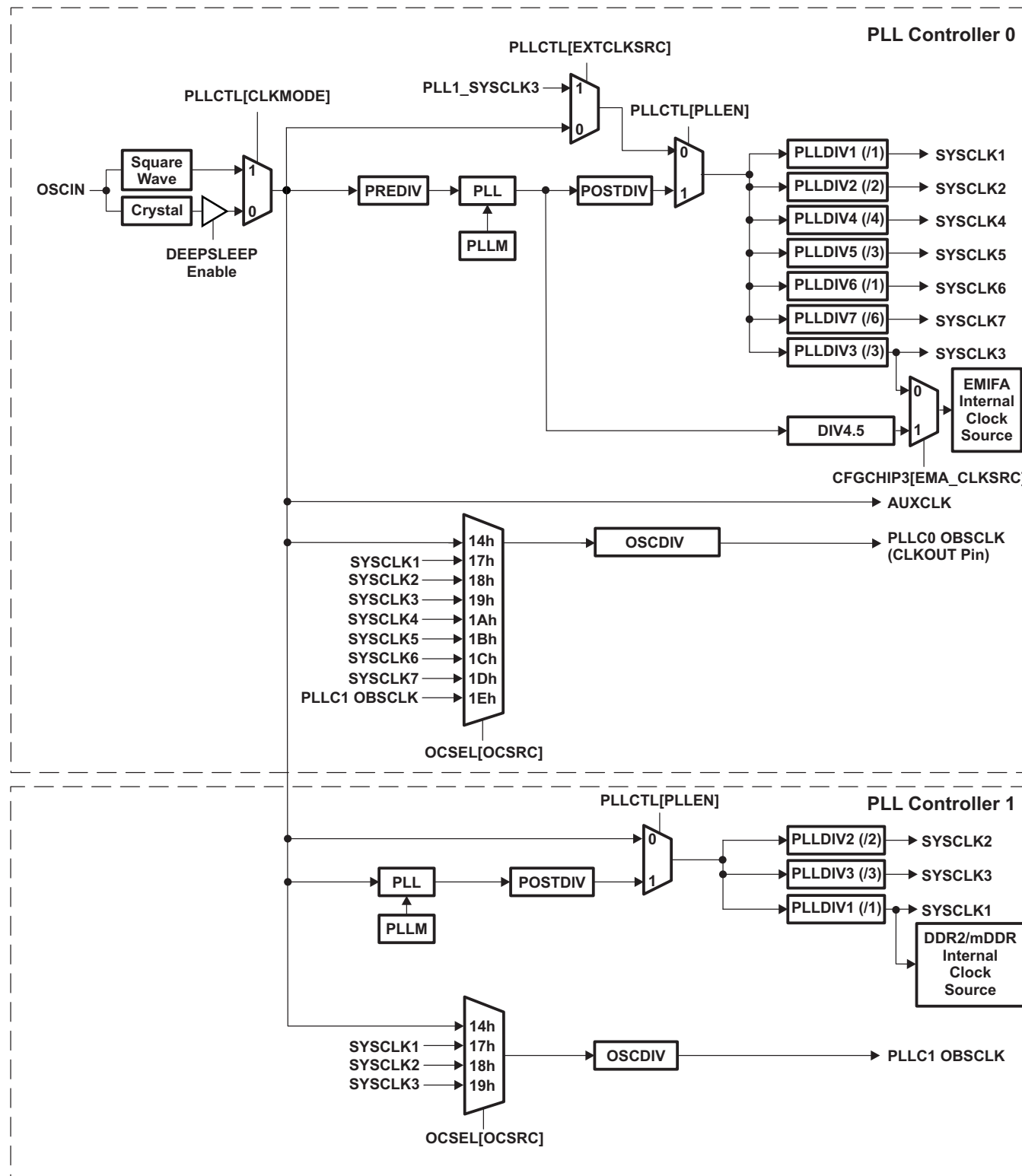
Figure 6-9. PLL Topology
