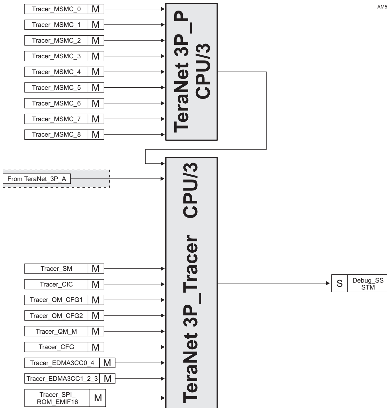
Figure 7-7. TeraNet 3P_Tracer
