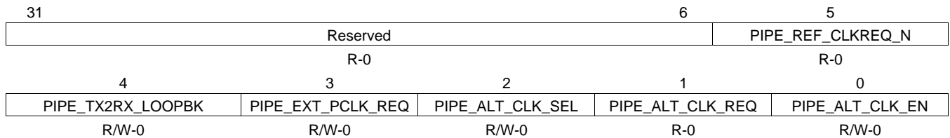
Figure 8-35. USB_PHY_CTL1 Register
