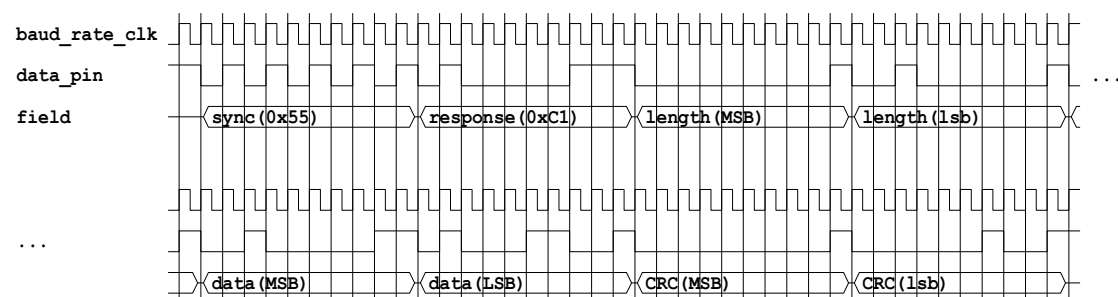
Figure 39-10. Example Response
