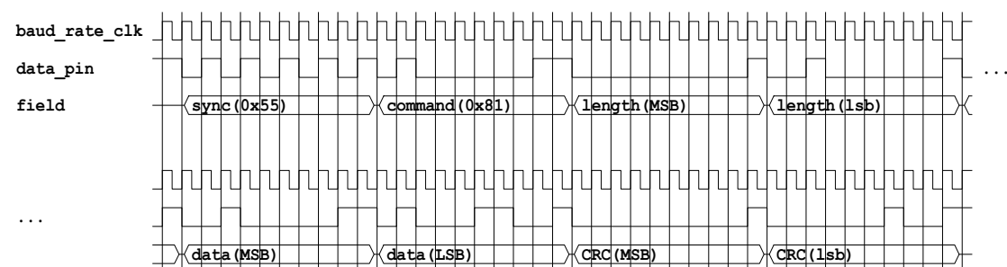
Figure 39-9. Example Command
