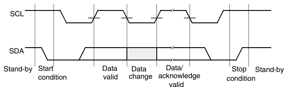
Figure 6-2. MCL Protocol
