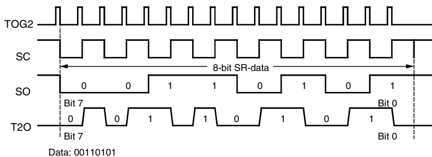
Figure 5-51. Manchester Modulation 1
