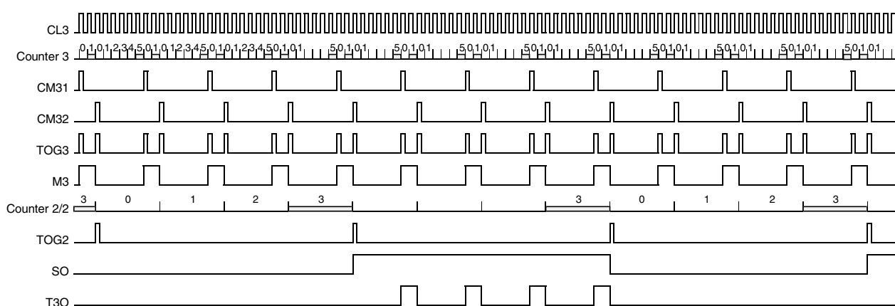
Figure 5-64. Burst Modulation 2
