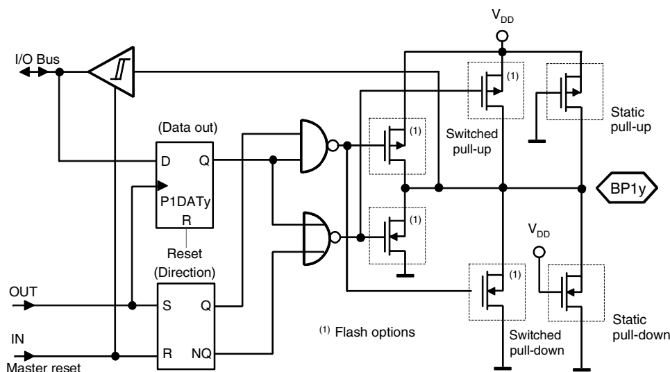
Figure 5-2. Bi-directional Port 1
