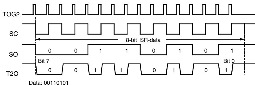
Figure 5-50. Bi-phase Modulation 1
