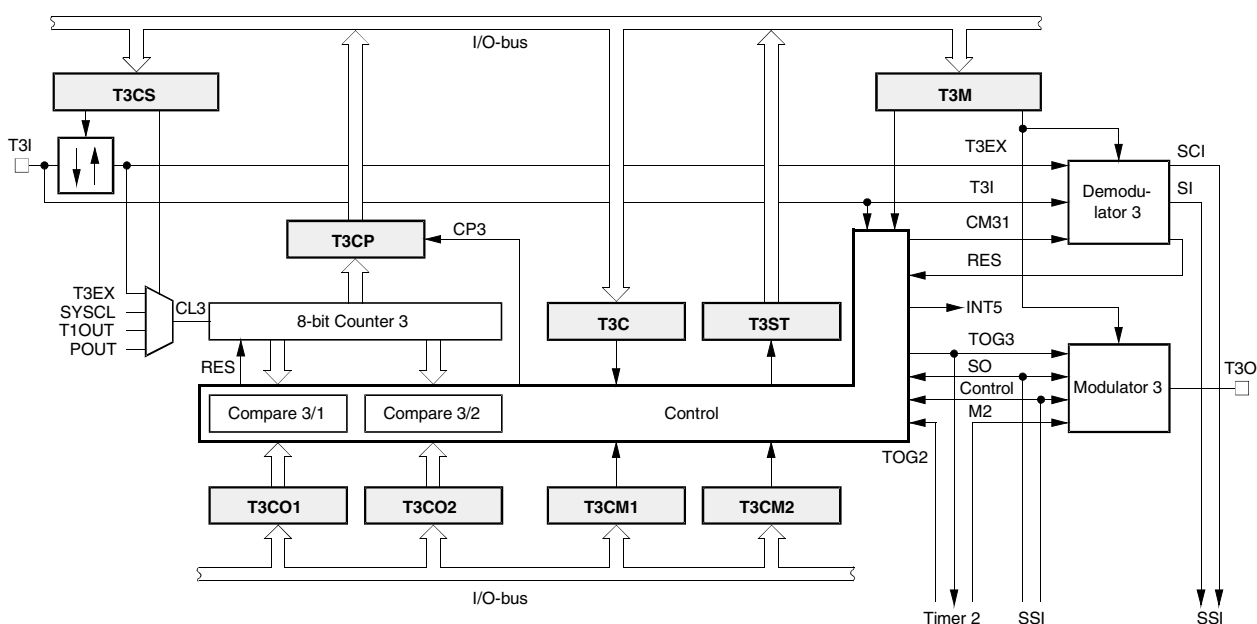
Figure 5-24. Timer 3
