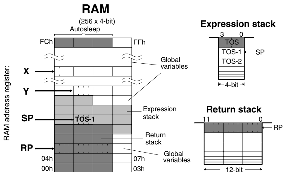
Figure 4-3. RAM Map
