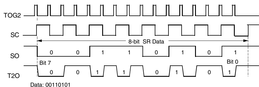
Figure 5-20. Bi-phase Modulation
