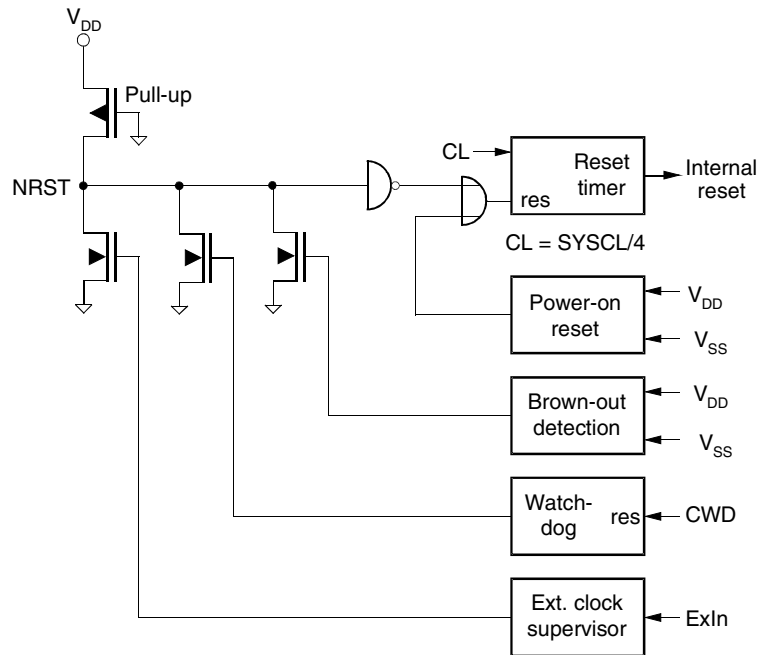
Figure 4-7. Reset Configuration
