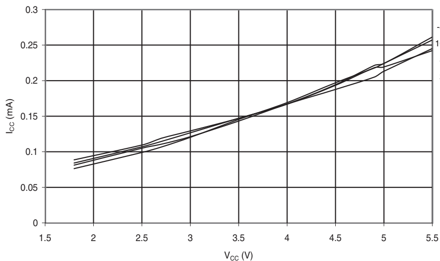
Figure 28-85. ATmega644P: Active Supply Current vs. V_{CC} (Internal RC Oscillator, 128 kHz)
