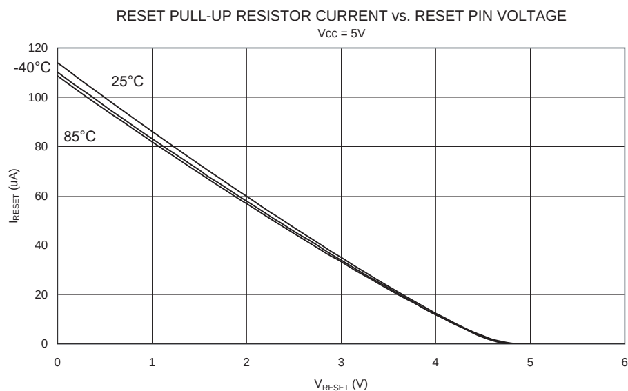
Figure 161. Reset Pull-up Resistor Current vs. Reset Pin Voltage ( V_{CC} = 5V )
