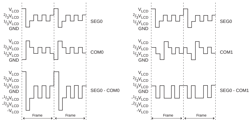
Figure 101. Driving a LCD with Four Common Terminals
