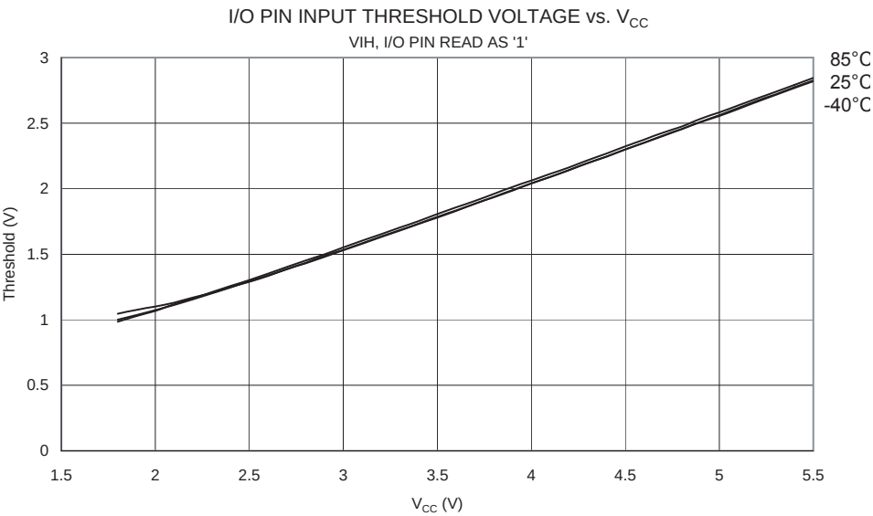
Pin Thresholds and hysteresis Figure 176. I/O Pin Input Threshold Voltage vs. V_{CC} ( V_{IH} , I/O Pin Read as “1”)
