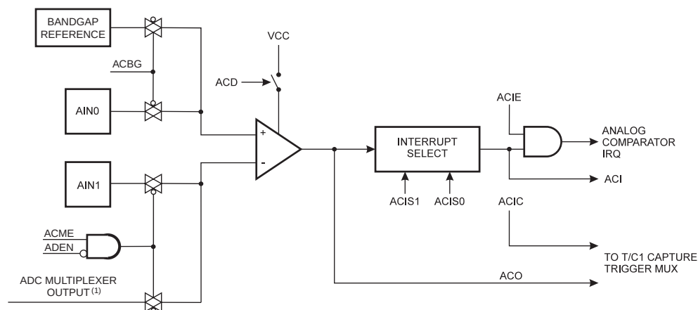
Figure 81. Analog Comparator Block Diagram (2)
