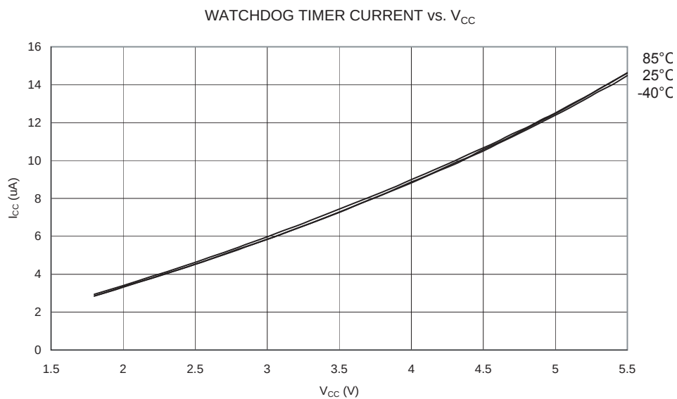
Figure 196. Watchdog Timer Current vs. V_{CC}
