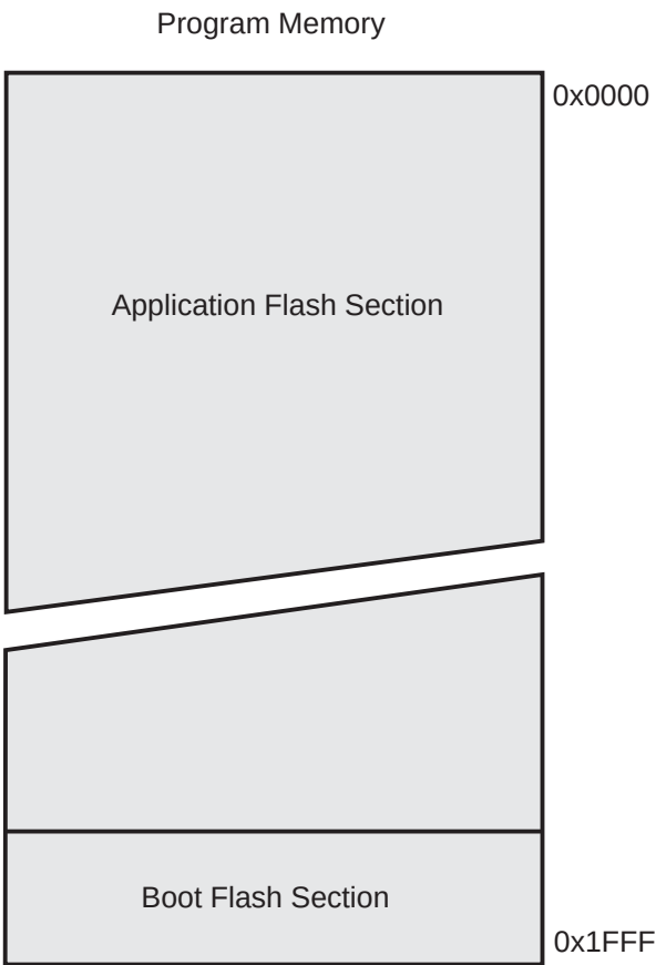
Figure 8. Program Memory Map
