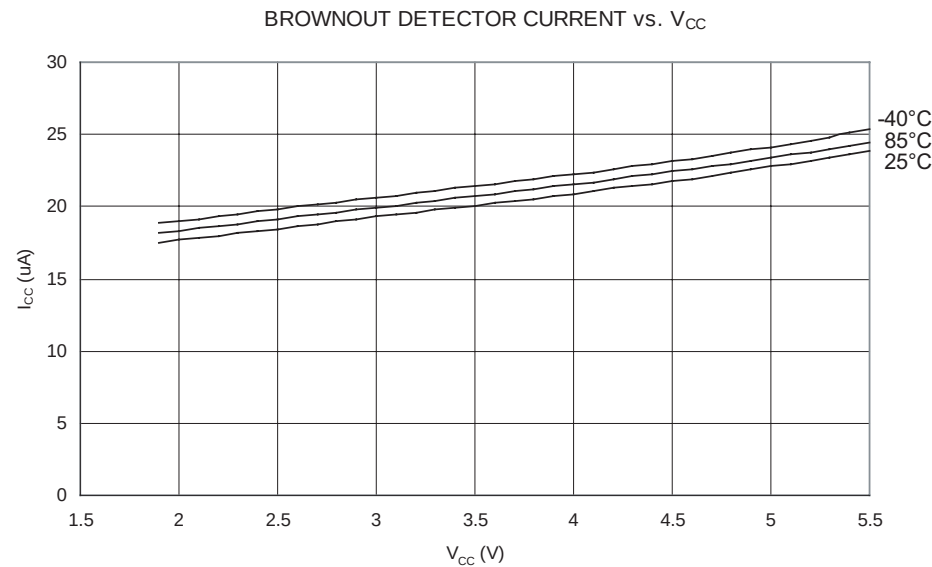
Figure 192. Brownout Detector Current vs. V_{CC}
