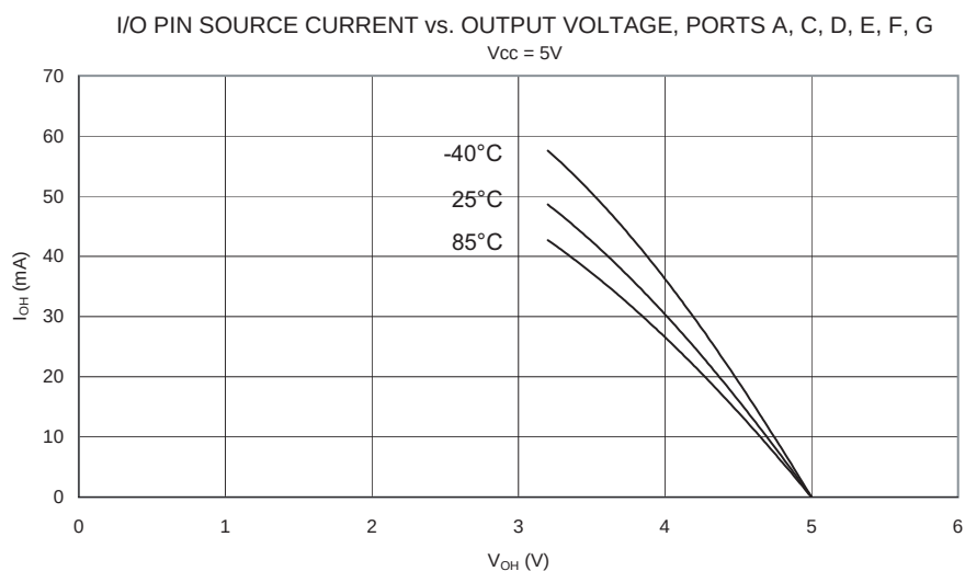
Figure 165. I/O Pin Source Current vs. Output Voltage, Ports A, C, D, E, F, G ( V_{CC} = 2.7V )
