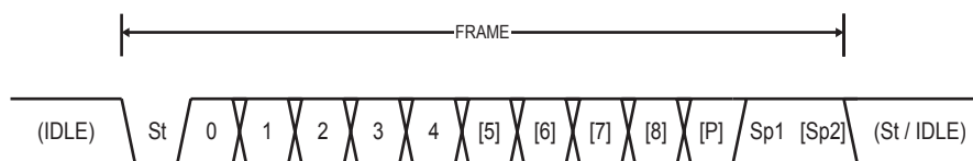
Figure 71. Frame Formats
