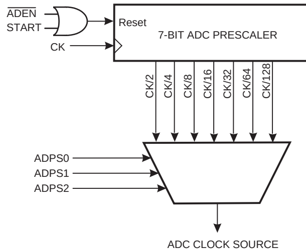
Figure 84. ADC Prescaler
