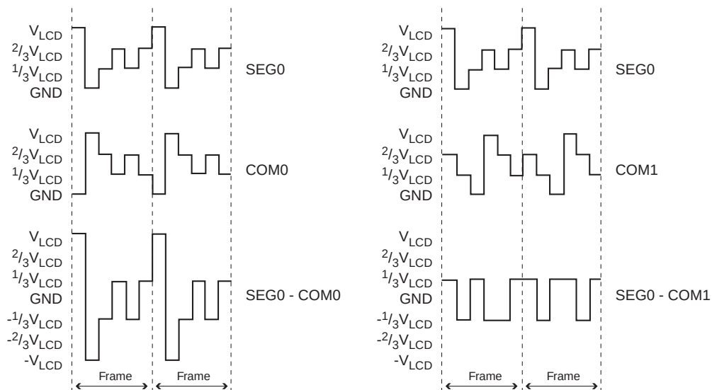
Figure 100. Driving a LCD with Three Common Terminals
