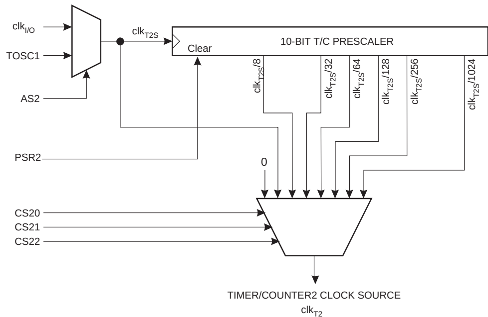
Figure 63. Prescaler for Timer/Counter2
