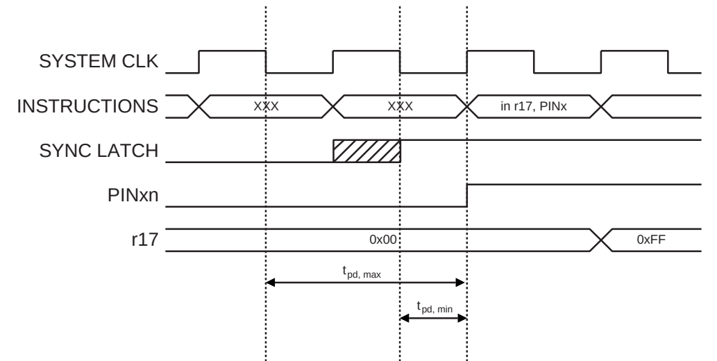
Figure 23. Synchronization when Reading an Externally Applied Pin value
