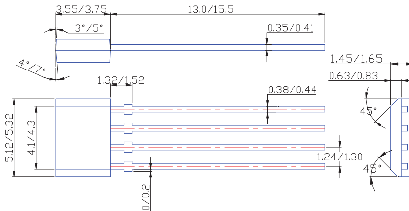
Package Dimension
