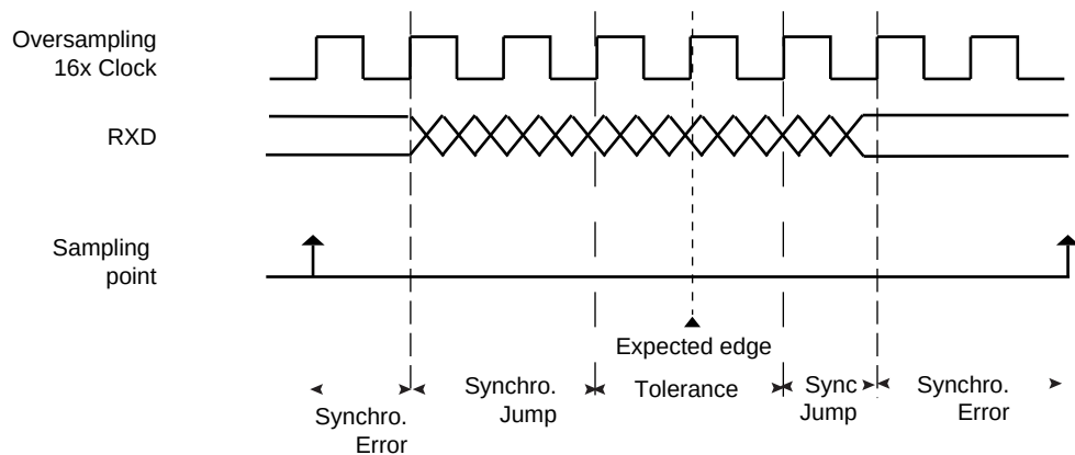
Figure 24-48. Bit Resynchronization
