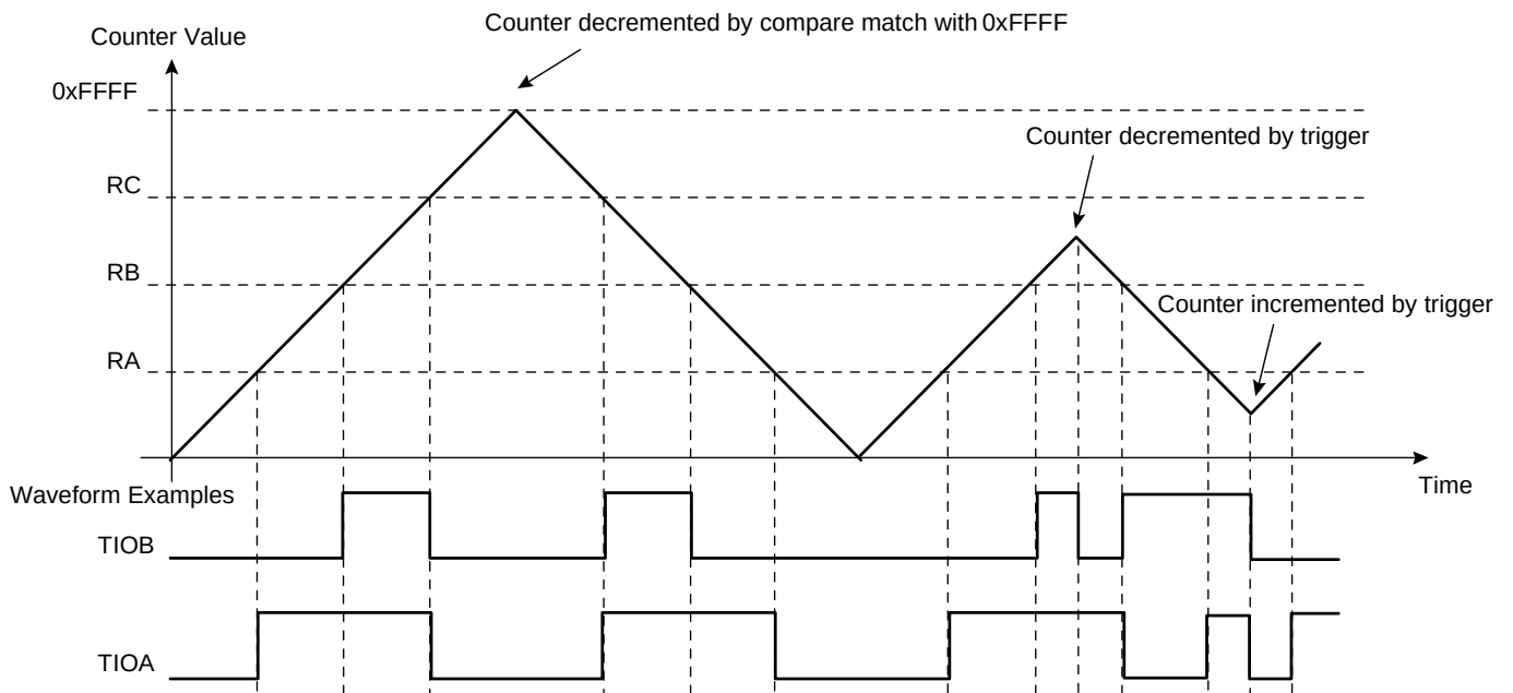
Figure 30-10. WAVSEL = 1 With Trigger
