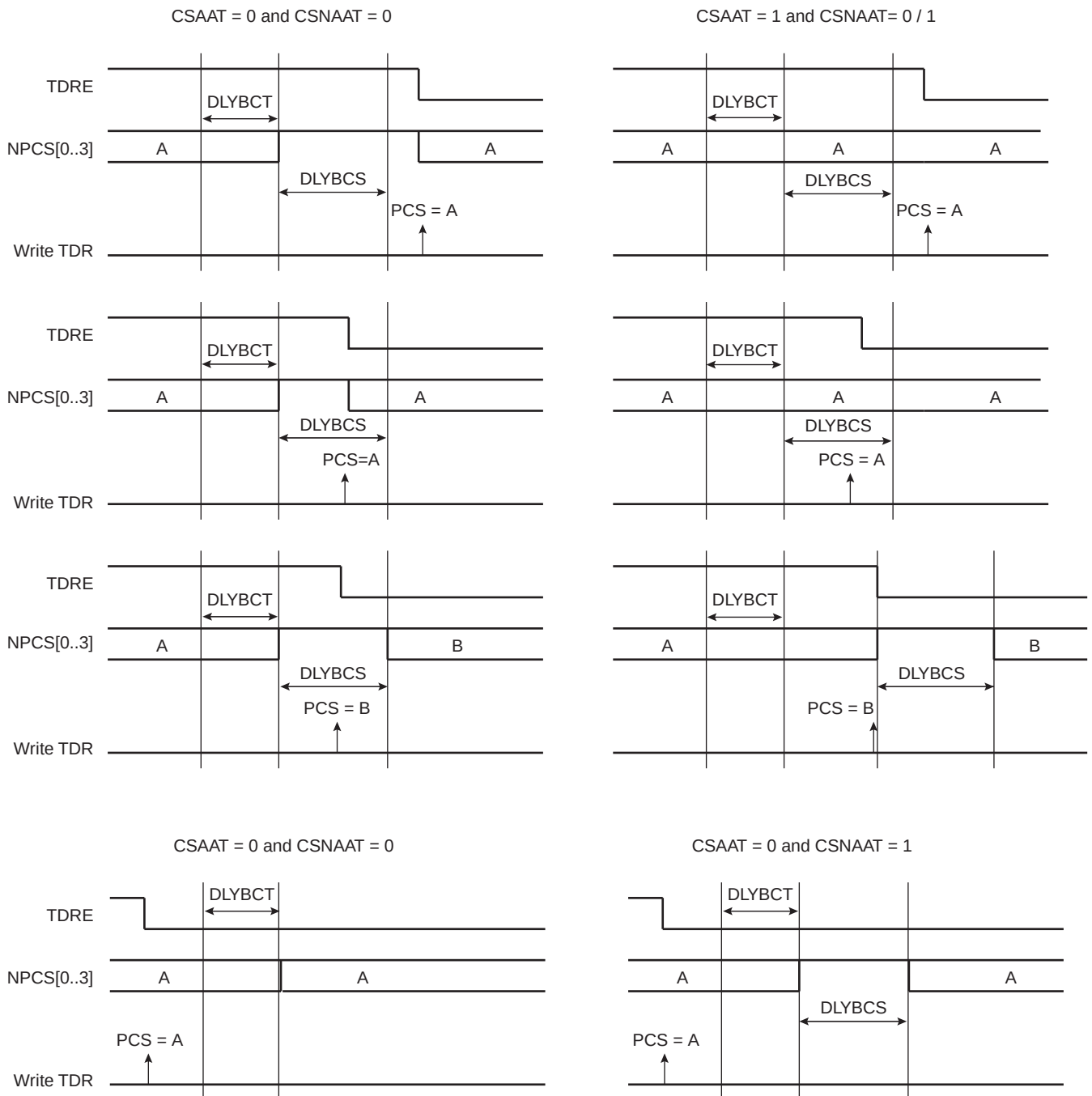
Figure 26-8. Peripheral Deselection
