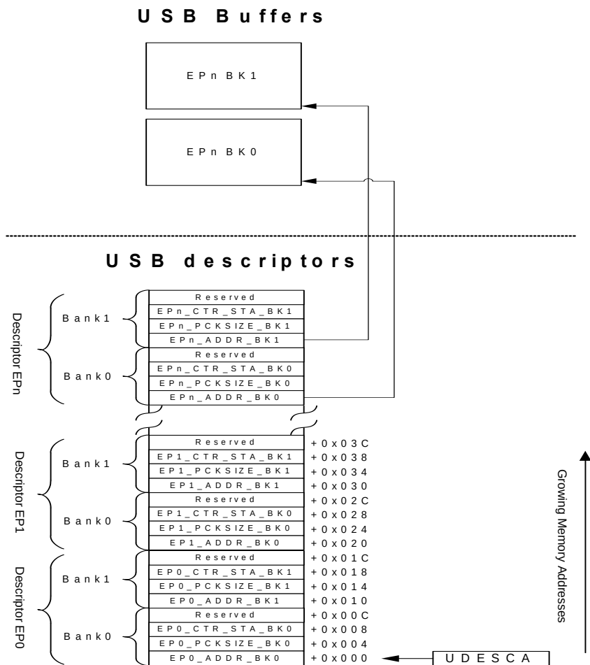
Figure 17-6. Memory organization
