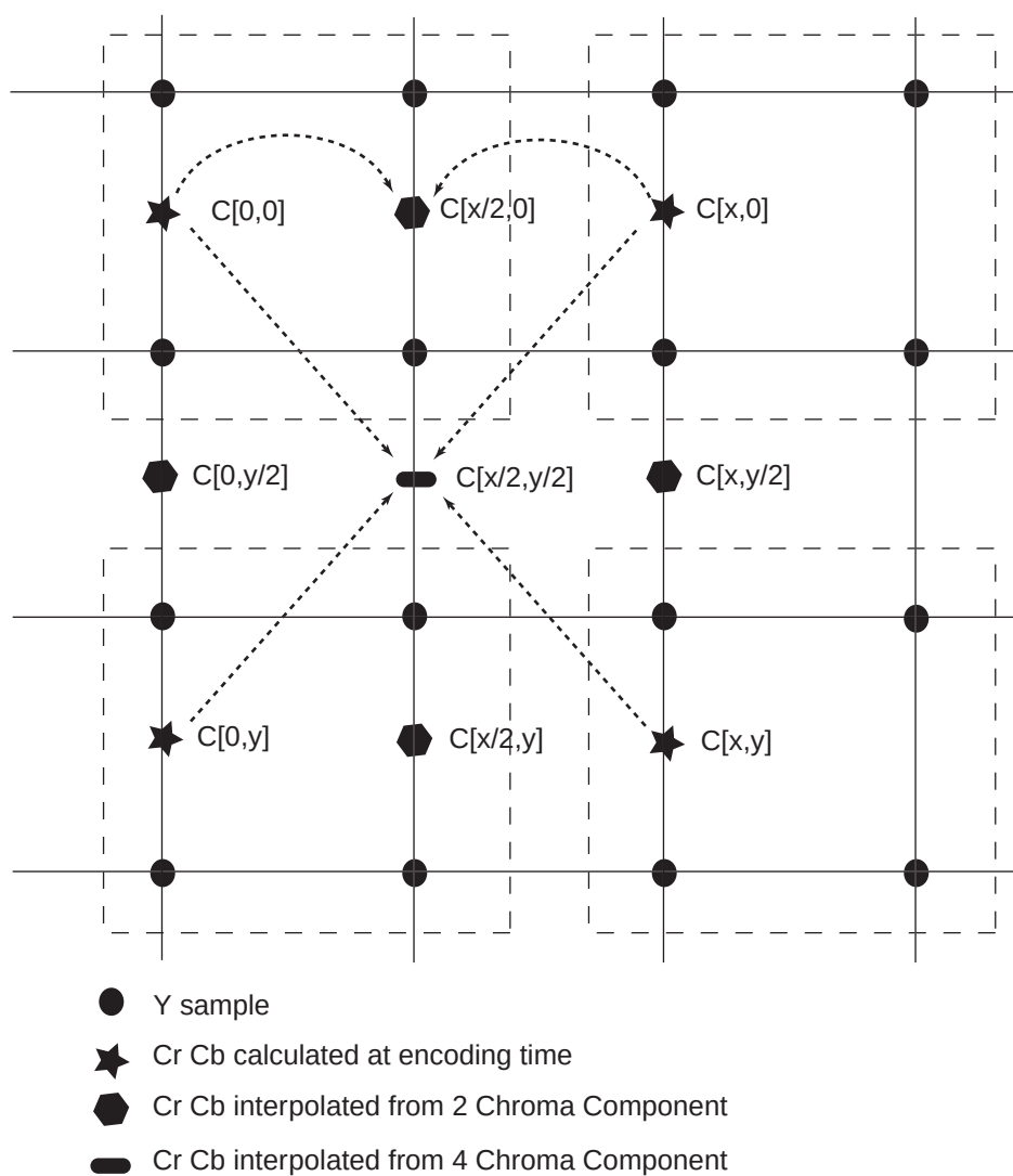
Figure 32-5. 4:2:0 Upsampling Algorithm
