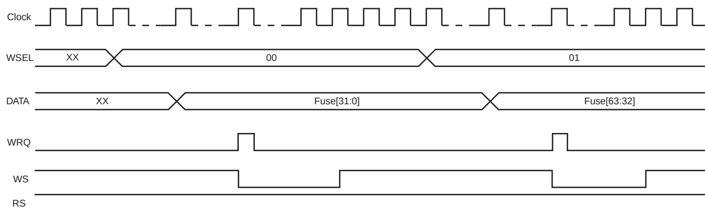
Figure 25-3. Fuse Write
