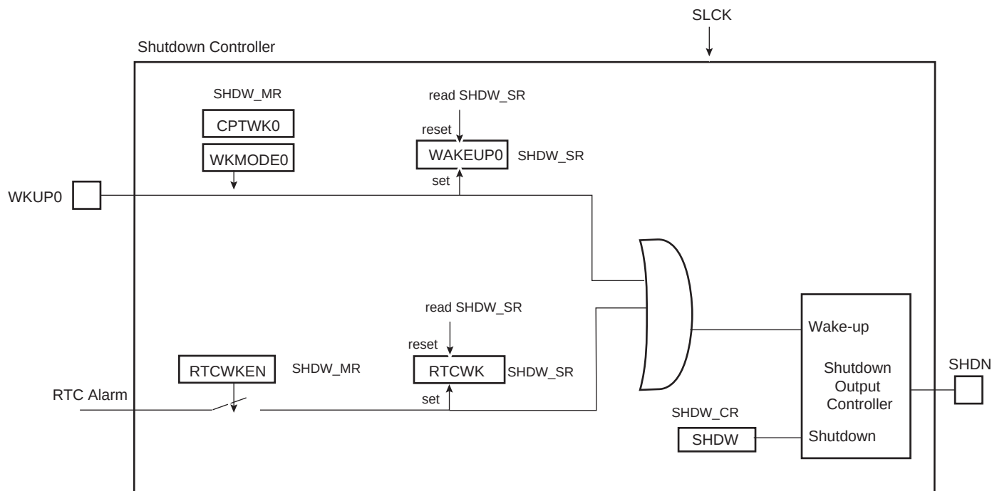
Figure 20-1. Shutdown Controller Block Diagram
