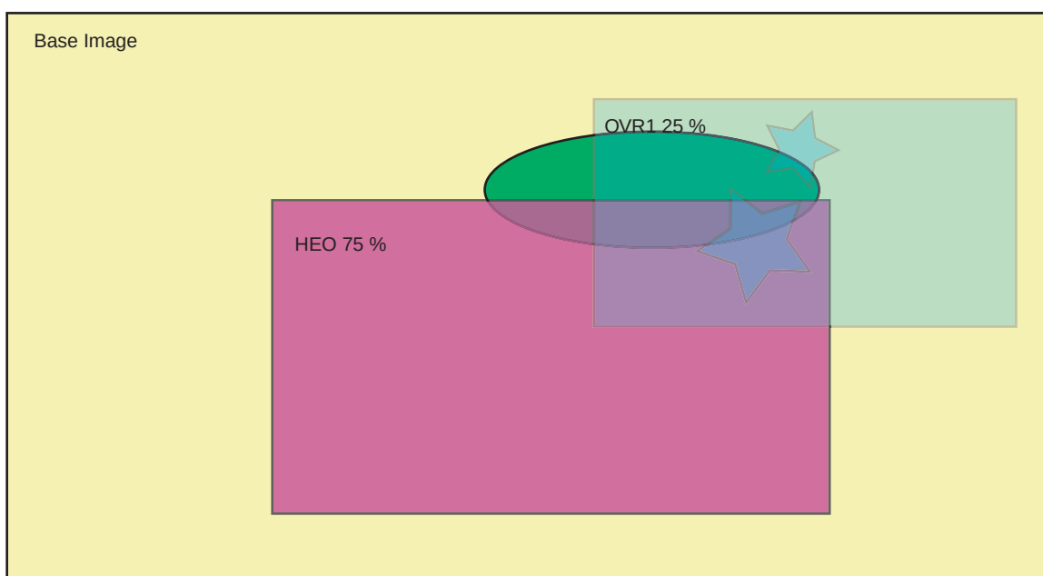
Figure 32-14.256-level Alpha Blending
