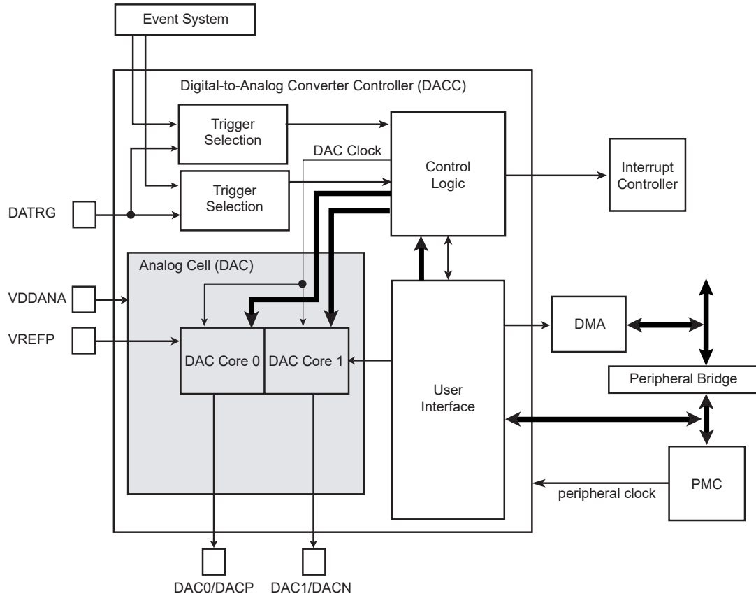
Figure 53-1. Block Diagram
