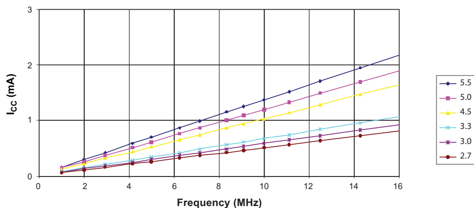
Figure 22-2. Idle Supply Current versus Frequency (0 - 16 MHz)
