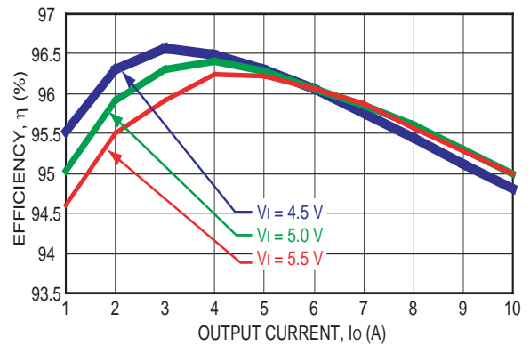
Figure 10. Converter Efficiency vs output current AXH010A0F-SR(3.3V Output Voltage).
