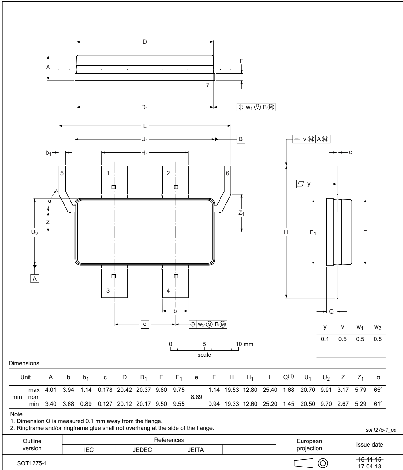
Fig 14. Package outline SOT1275-1
