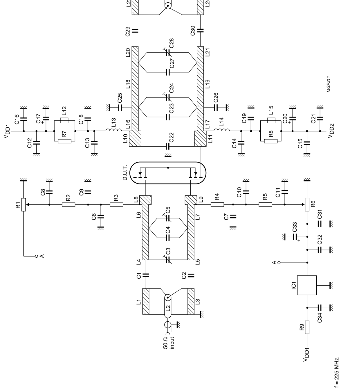
Fig.11 Test circuit for class-AB operation.
