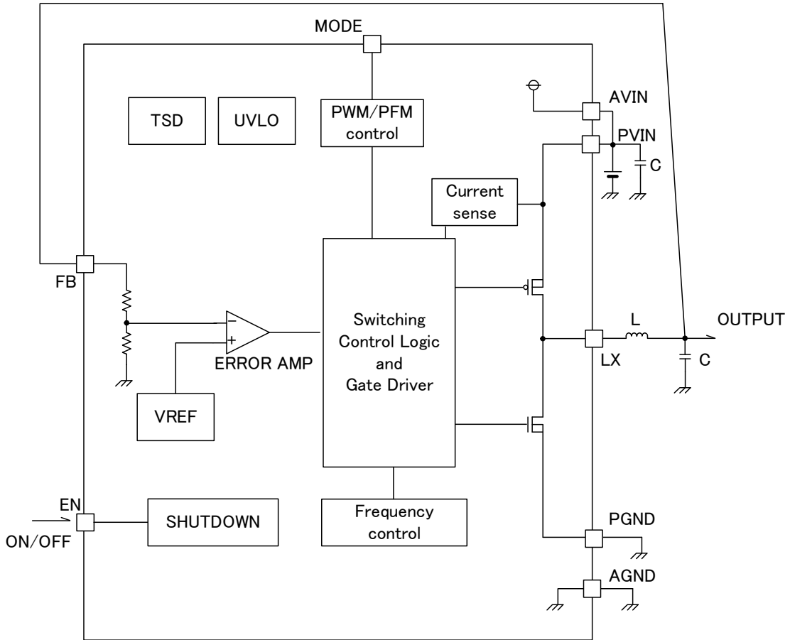
Figure 3. Block Diagram(s)
