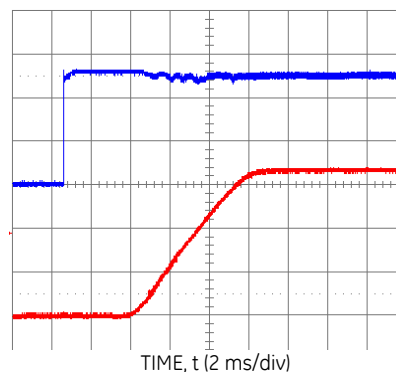
Figure 16. Typical Start-Up with application of V_{in} ( V_{in} = 5.0\text{Vdc} , V_o = 3.3\text{Vdc} , I_o = 6\text{A} ).
