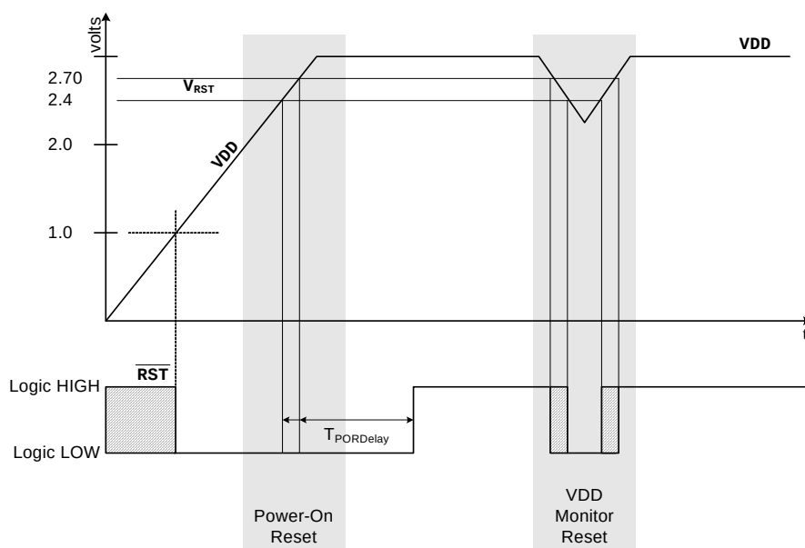
Figure 11.2. Power-On and V_{DD} Monitor Reset Timing
