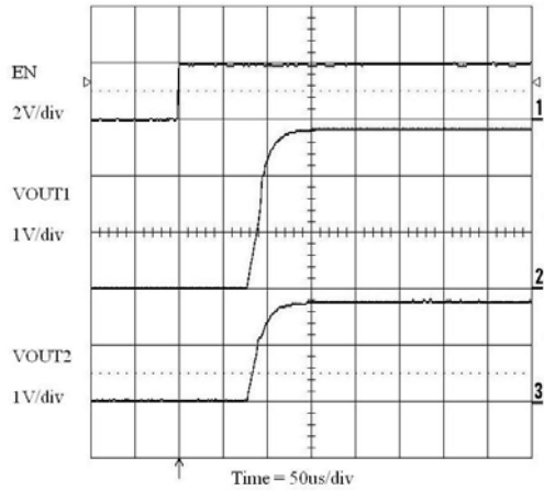
Figure 18. Enable Turn-on (100 \mu\text{A} Loads)
