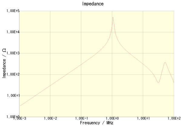
CLF12555T-471M-CA
