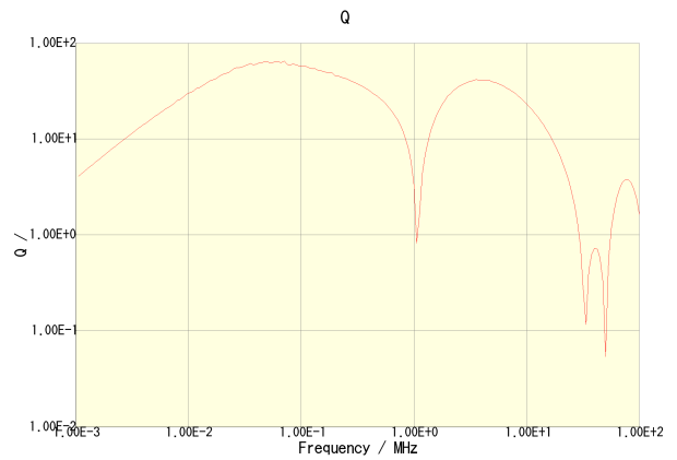
CLF12555T-471M-CA
