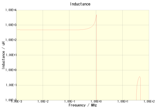
CLF12555T-471M-CA
