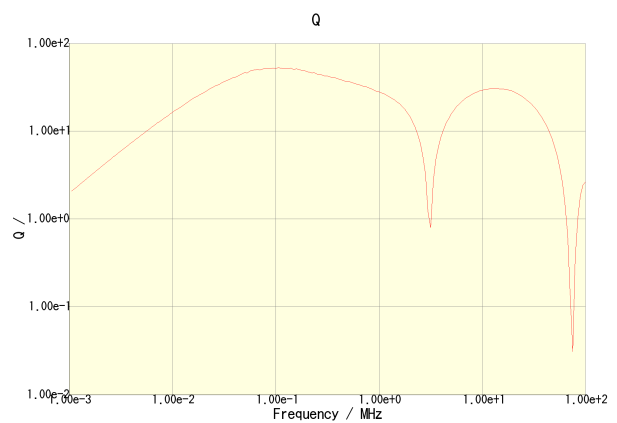
CLF6045T-151M-CA
