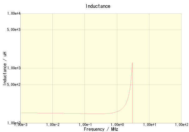
CLF6045T-151M-CA
