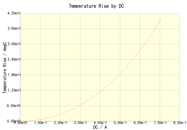
CLF6045T-151M-CA(Amb. Temp. = 20degc)
