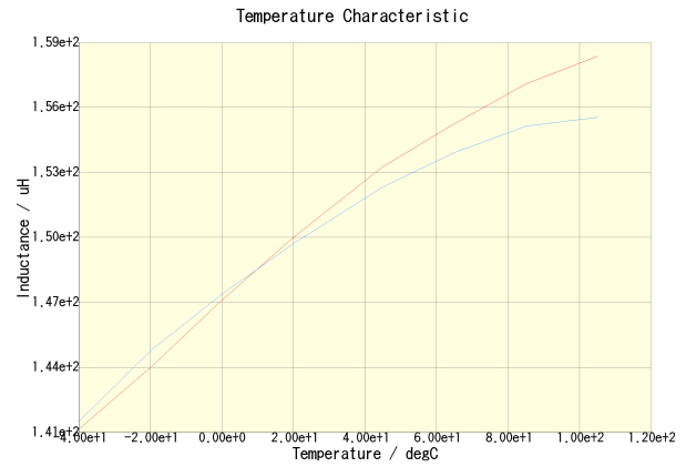
CLF6045T-151M-CA(DC = 0A)
