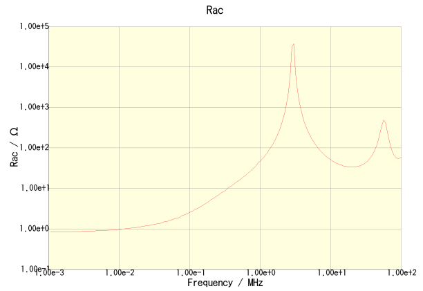
CLF6045T-221M-CA
