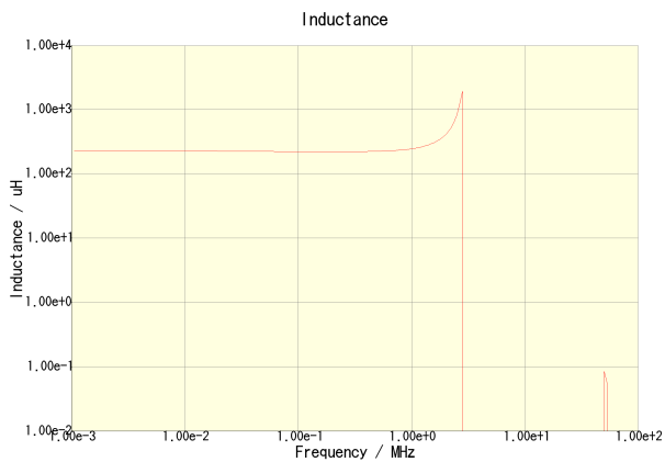
CLF6045T-221M-CA
