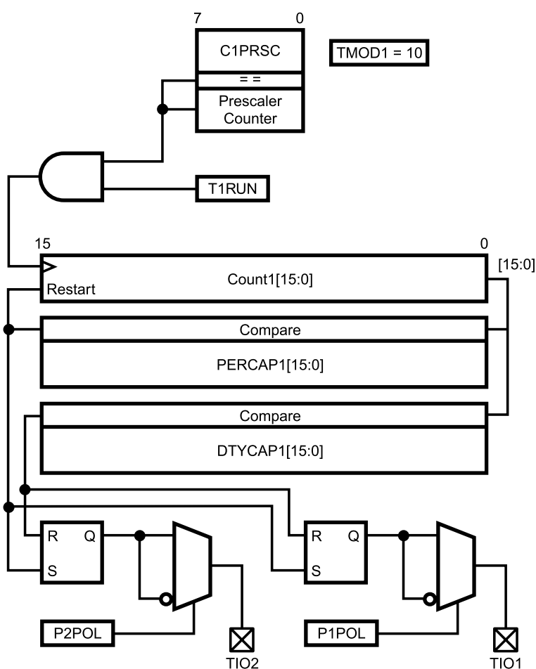
Figure 23-4. VTU 16-bit PWM Mode
