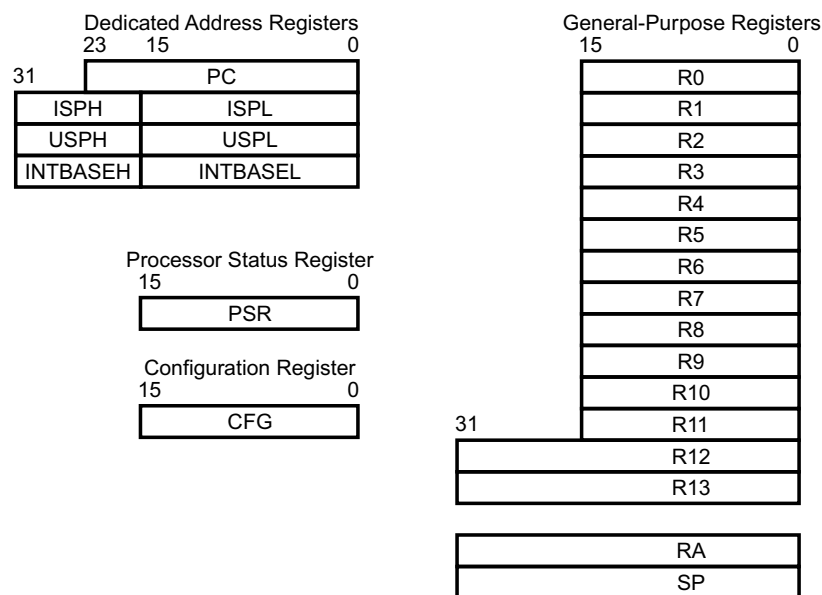
Figure 5-1. CPU Registers
