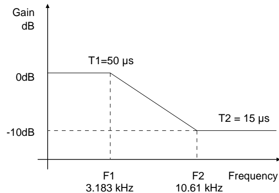
Figure 6. De-Emphasis Curve
