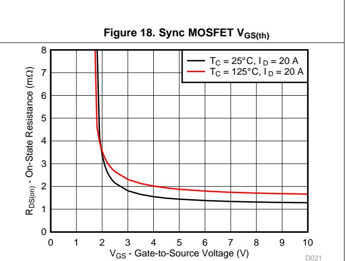
Figure 20. Sync MOSFET R_{DS(on)} vs V_{GS}
