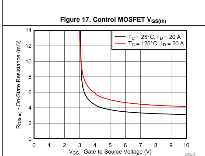
Figure 19. Control MOSFET R_{DS(on)} vs V_{GS}
