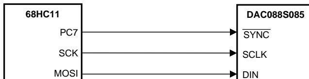
Figure 36. 68HC11 Interface
