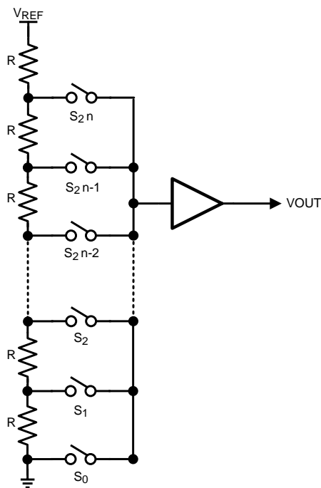
Figure 27. DAC Resistor String
