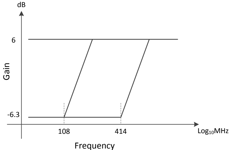
Figure 37. Equalizer Frequency Response
