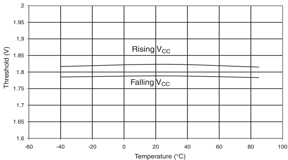
Figure 26-33. BOD Threshold vs. Temperature (Bodlevel is 1.8V).
