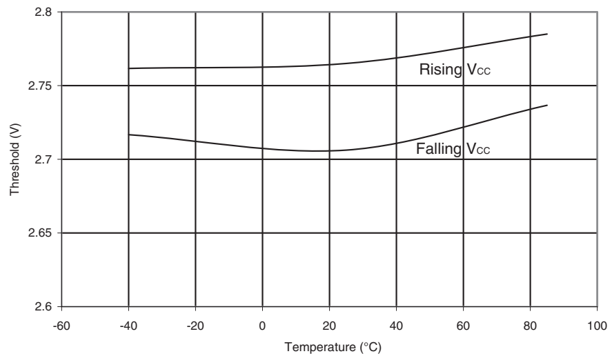
Figure 26-126. BOD Threshold vs. Temperature ( V_{CC} = 2.7V )
