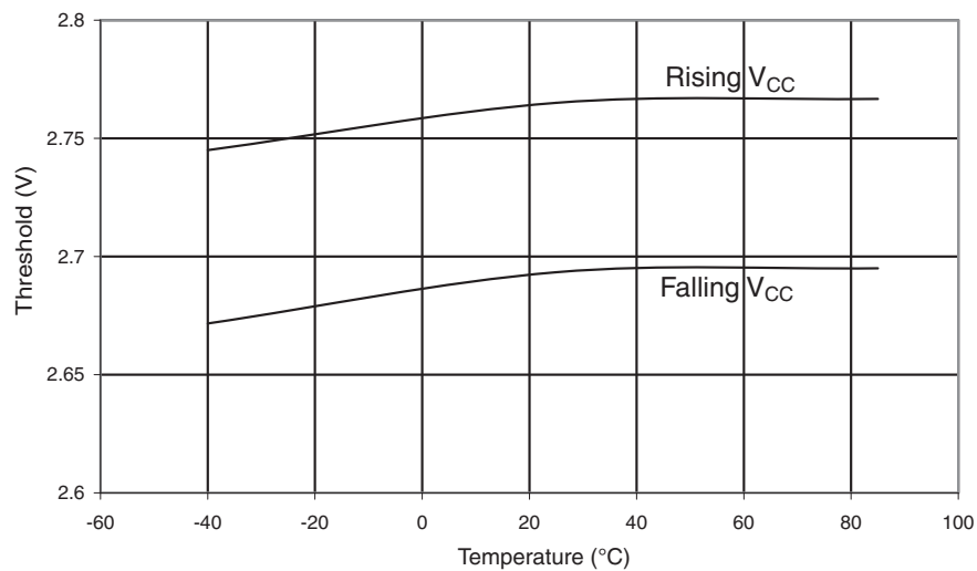
Figure 26-79. BOD Threshold vs. Temperature ( V_{CC} = 2.7V )
