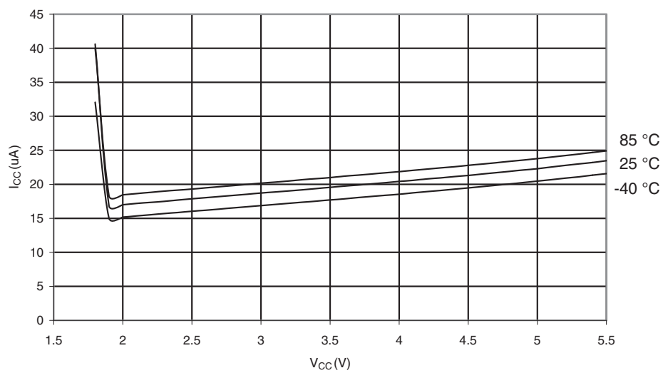
Figure 26-136. Brownout Detector Current vs. V_{CC}
