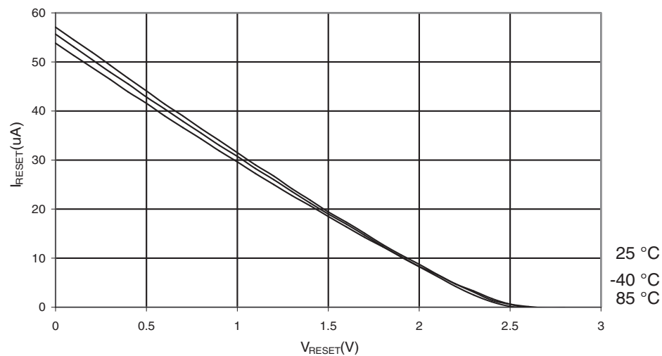
Figure 26-19. Reset Pull-up Resistor Current vs. Reset Pin Voltage ( V_{CC} = 2.7V ).
