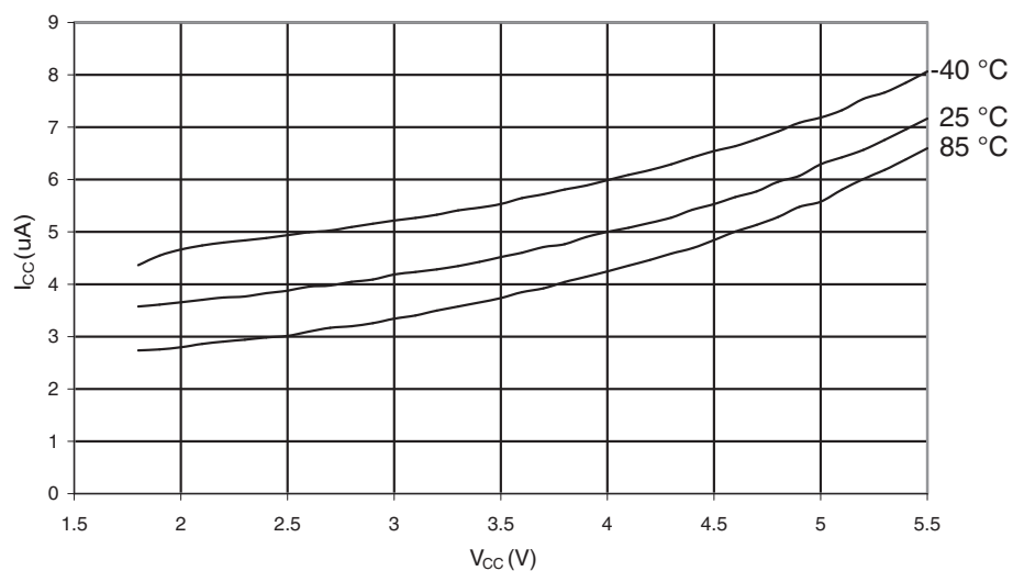
Figure 26-91. Watchdog Timer Current vs. V_{CC}
