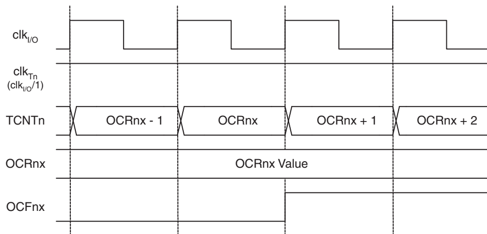
Figure 13-10. Timer/Counter Timing Diagram, Setting of OCF n , no Prescaling
