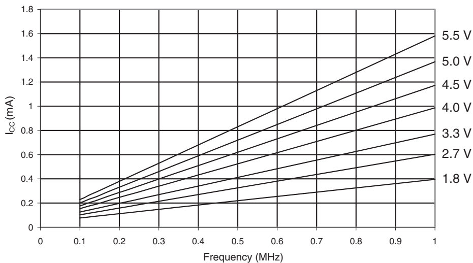
Figure 26-48. Active Supply Current vs. Low Frequency (0.1 - 1.0 MHz).
