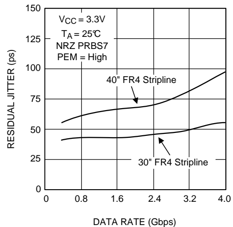
Figure 20. Residual Jitter as a Function of Data Rate, FR4 Stripline Length and PE Level
